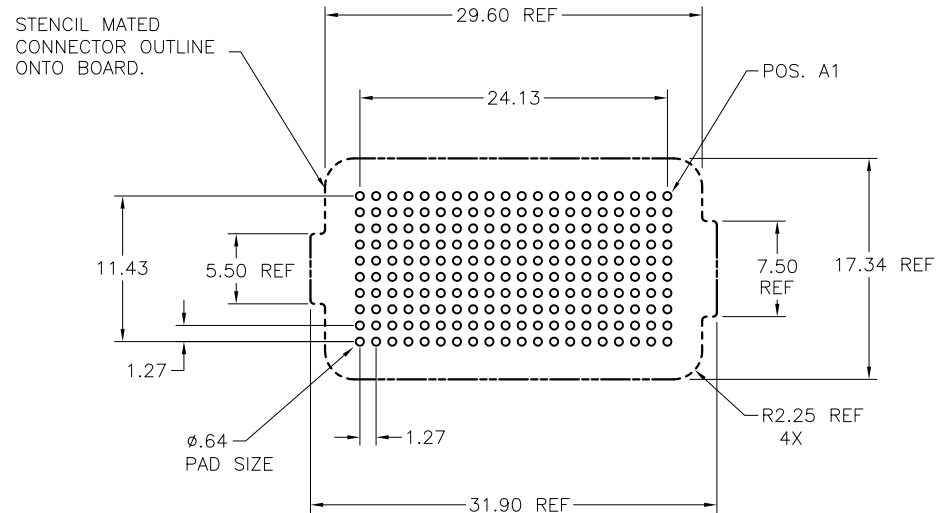
BOARD PATTERN
