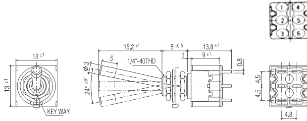
Terminal numbers are not shown on the switch.
