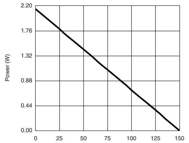
Power, Junction-to-Ambient
