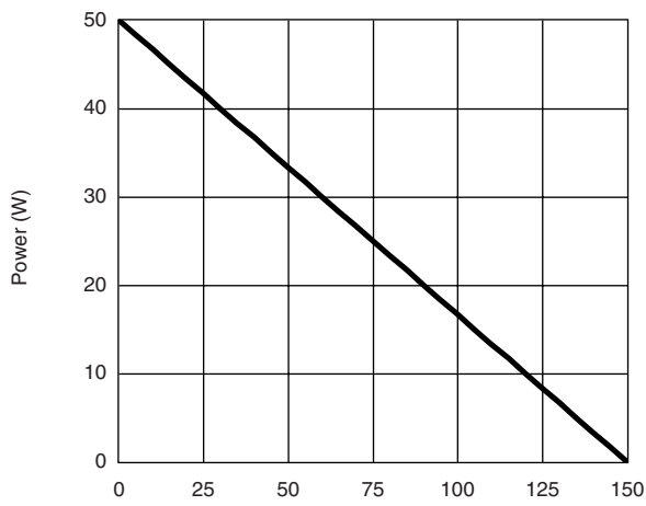
Power, Junction-to-Case
