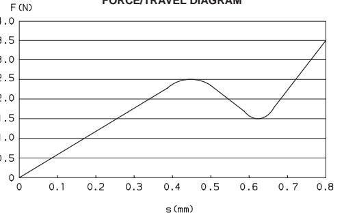
FORCE/TRAVEL DIAGRAM
